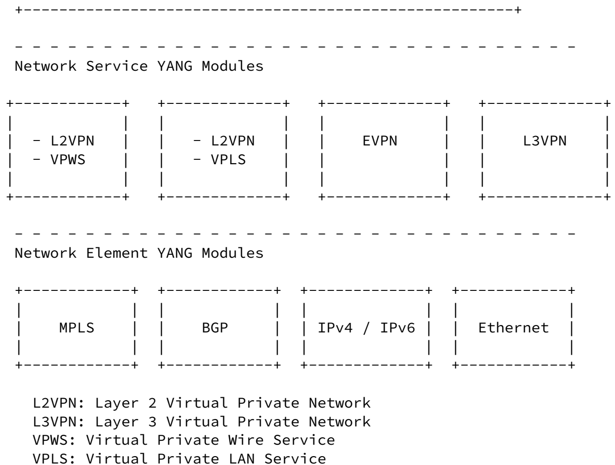
Figure 4: YANG Module Layers Showing Service Models
