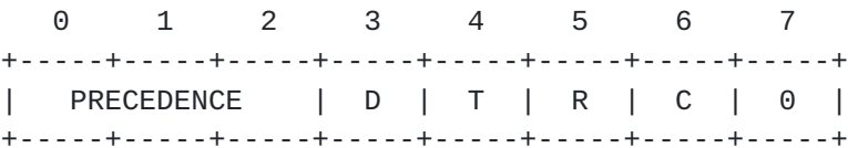
Figure 2: Type of Service Field (Original Interpretation)
