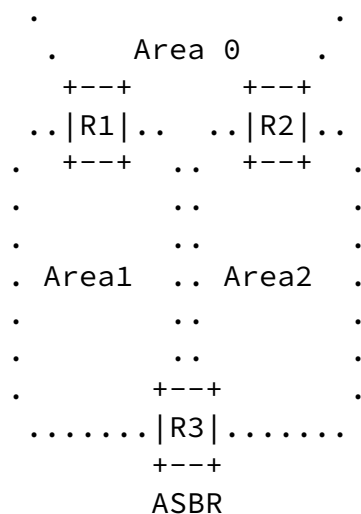
Customer Networks Advertised as AS External or NSSA External Routes
