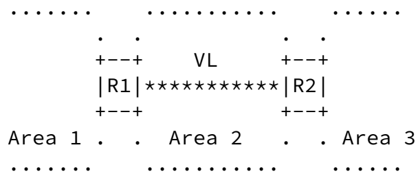
Figure 3. Purely Virtual Backbone
