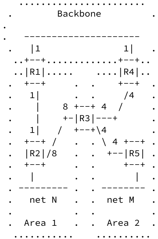
Figure 4. Inter-area routing asymmetry
