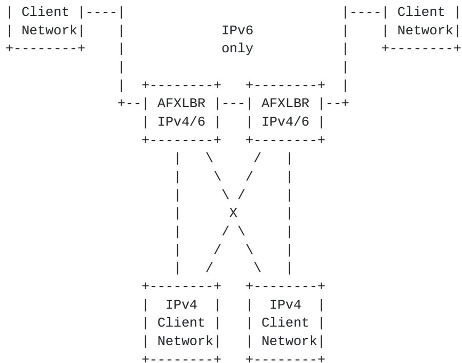
Figure 1: Segregated IPv4 Networks Inter-connected by an IPv6 Network
