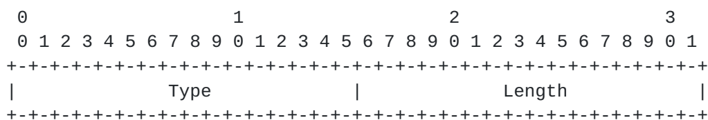
Figure 2: Link Overload sub-TLV for OSPFv3
