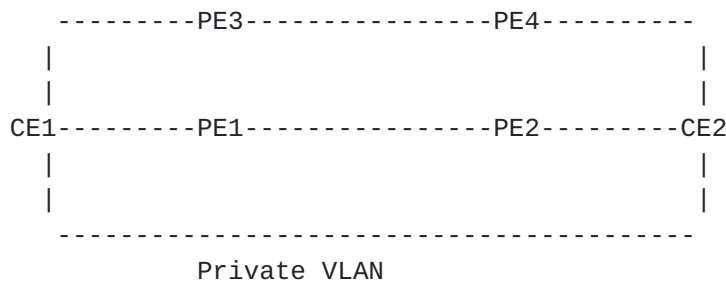
Figure 3: Pseudowire Services
