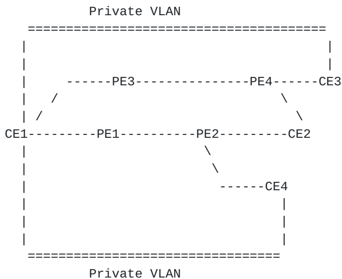
Figure 3: Pseudowire Services
