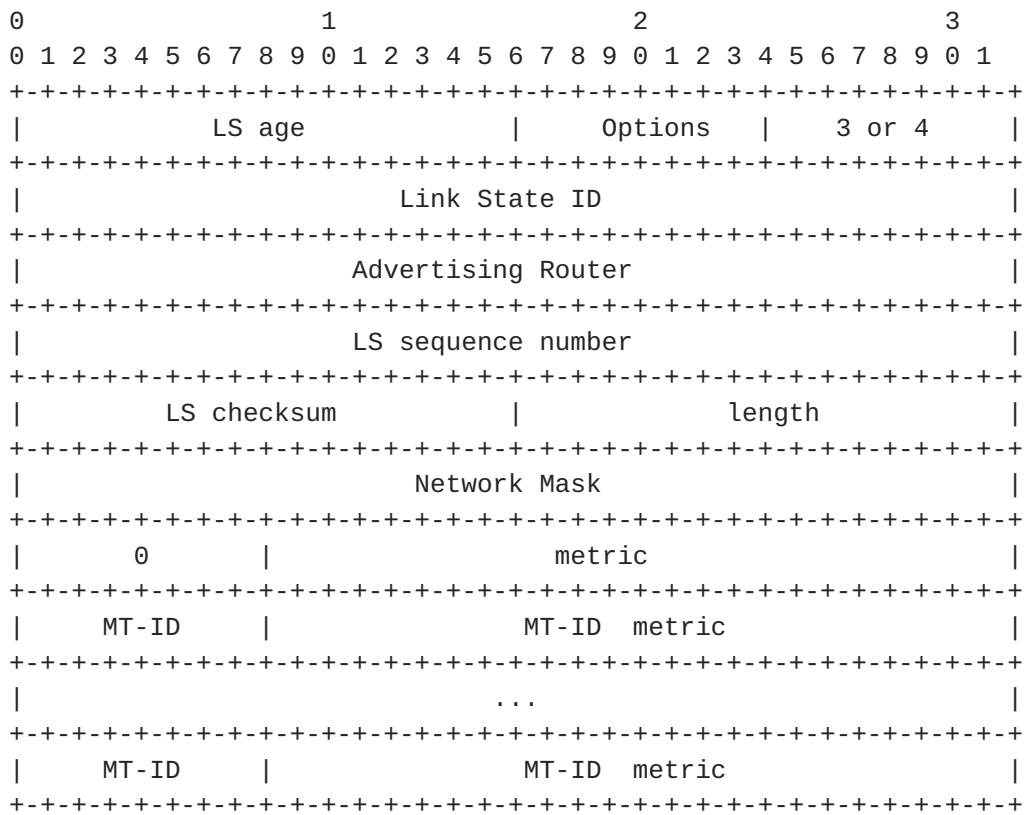
Figure 4: Summary-LSA Format
