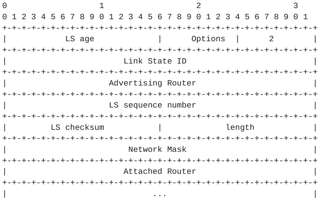
Figure 3: Network-LSA Format
