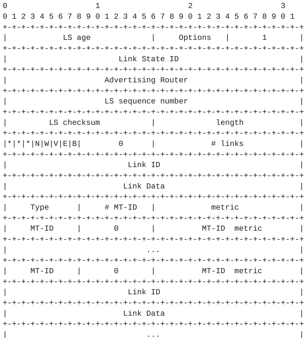
Figure 2: Router-LSA Format
