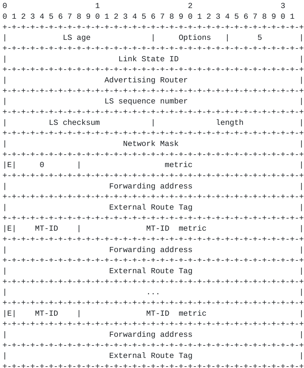
Figure 5: AS-External-LSA Format
