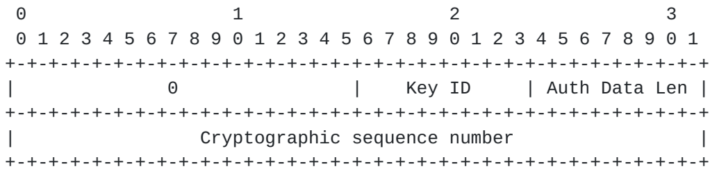
Figure 18: Usage of the Authentication field in the OSPF packet header when Cryptographic Authentication is employed
