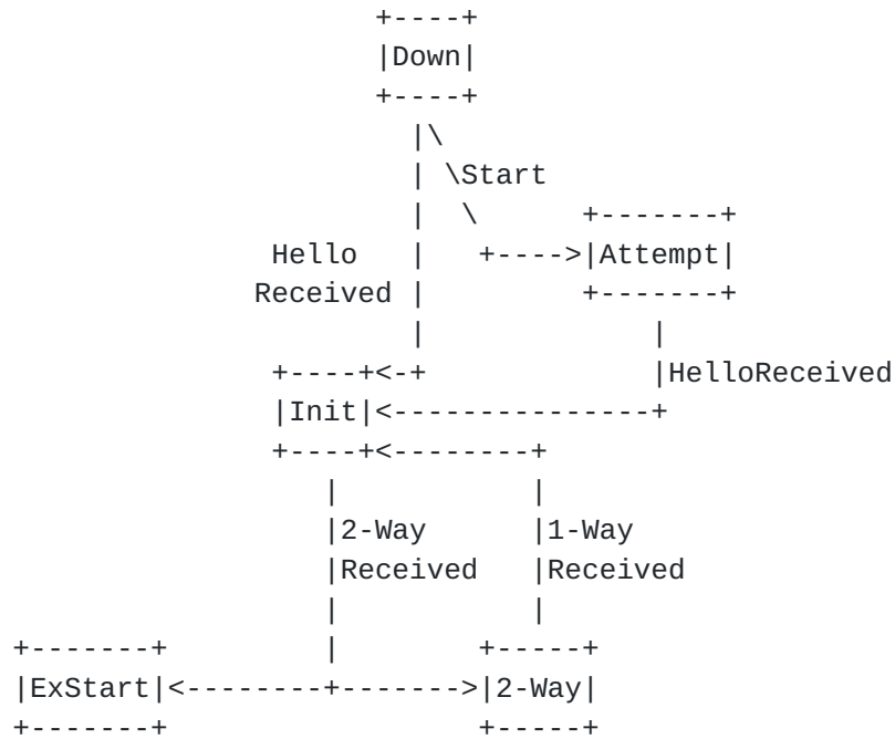
Figure 12: Neighbor state changes (Hello Protocol)
