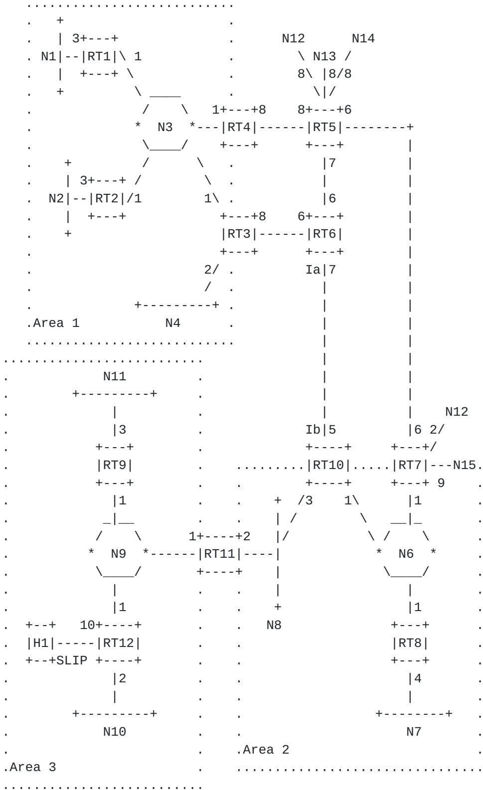
Figure 6: A sample OSPF area configuration
