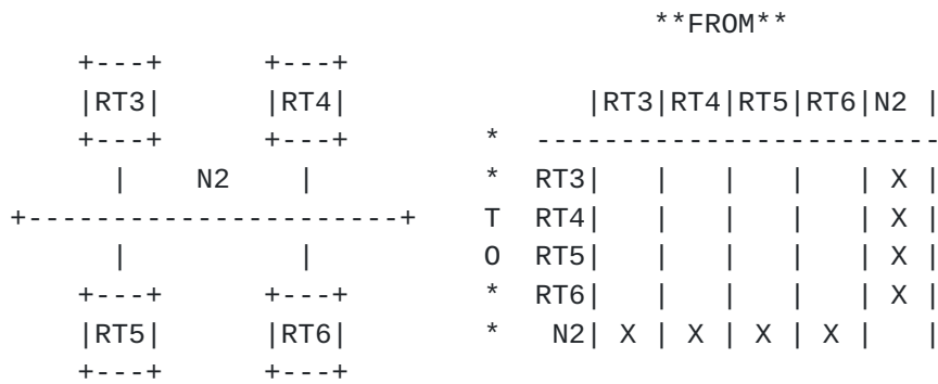
Broadcast or NBMA networks
