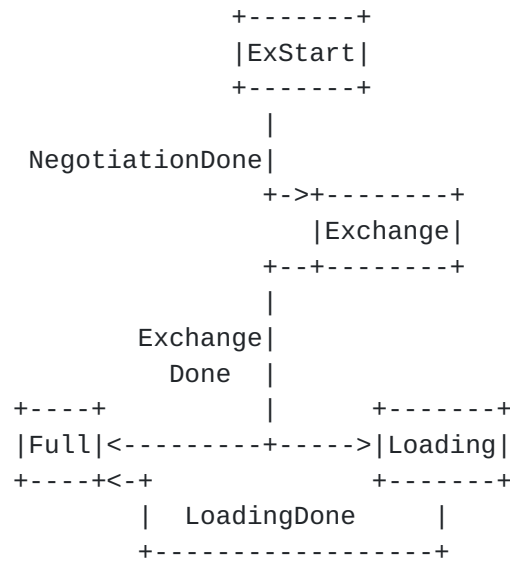
Figure 13: Neighbor state changes (Database Exchange)
