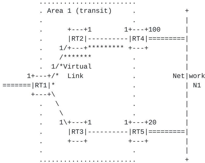
Figure 17: Routing through transit areas
