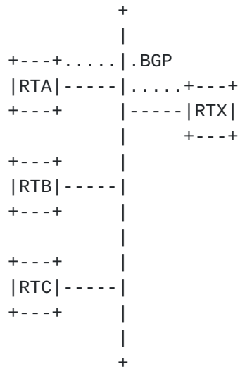
Figure 16: Forwarding address example
