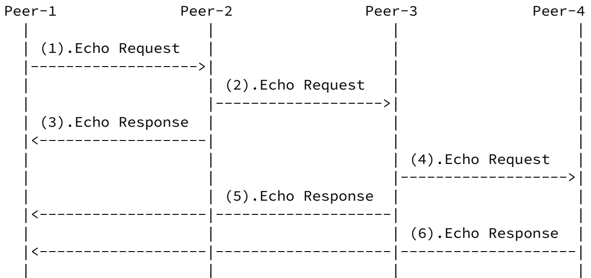
P2PSIP Echo example
