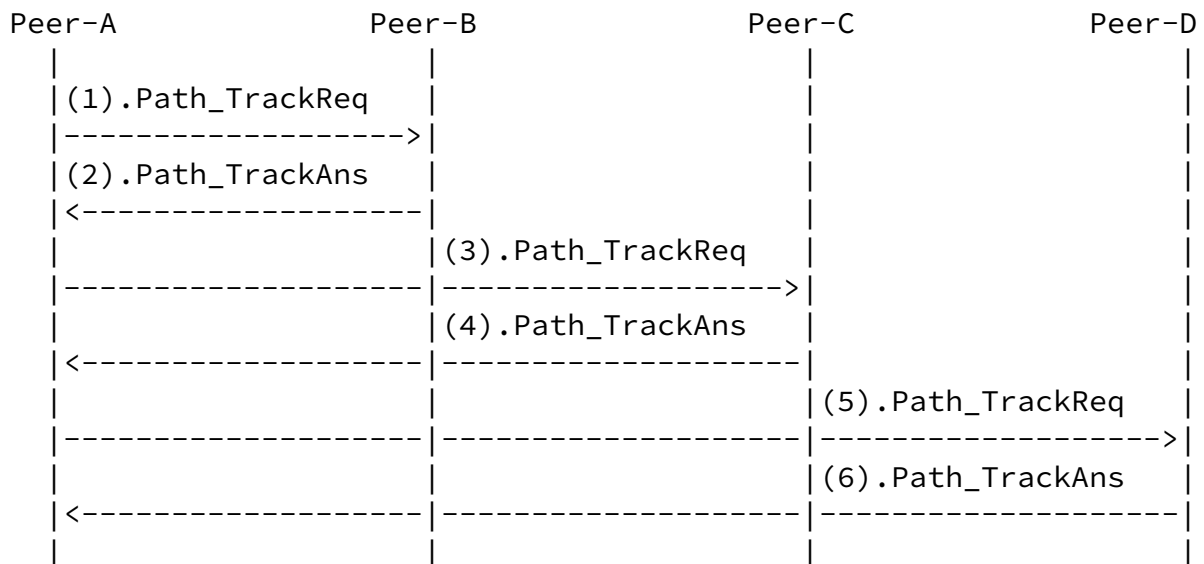
Path_Track Diagnostic Message Flow
