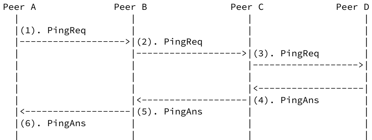
Ping Diagnostic Message Flow
