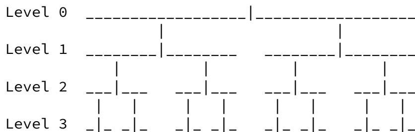
Figure 1: ReDiR tree
