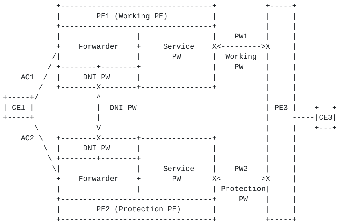
Figure 5. Components of one-side dual-homing PW protection
