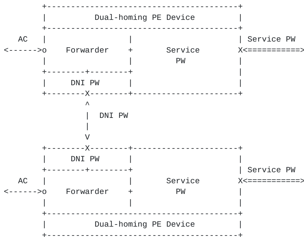
Figure 1: PE Architecture for Dual-homing Protection
