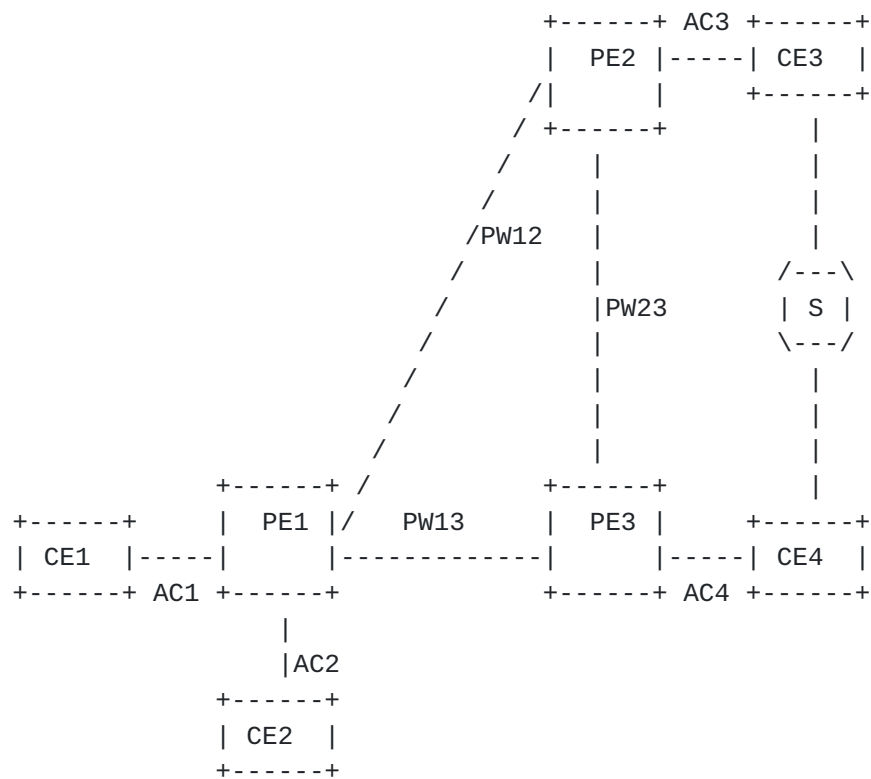
Figure 3: An Example Network for Triggering Assert
