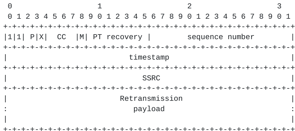
Figure 15: Protocol format for Retransmission
