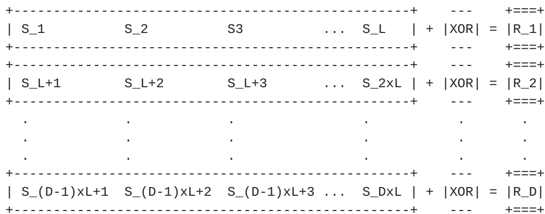
Figure 3: Generating non-interleaved (row) FEC packets
