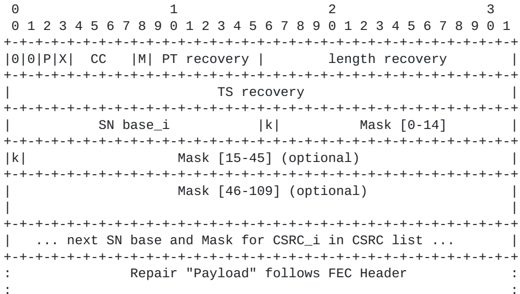
Figure 12: FEC Header for F=0
