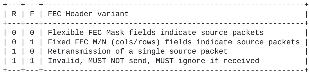
Figure 11: R and F bit values for FEC Header variants
