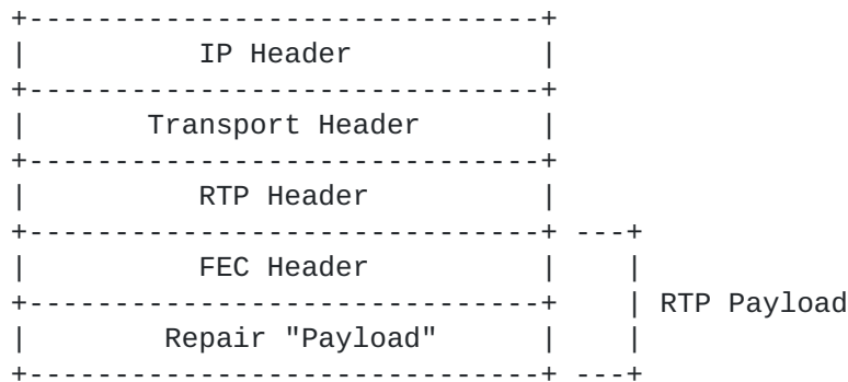
Figure 9: Format of FEC repair packets
