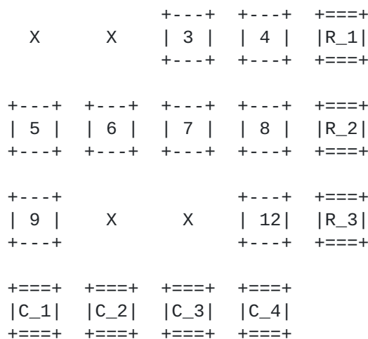
Figure 16: Example loss pattern for the iterative decoding algorithm
