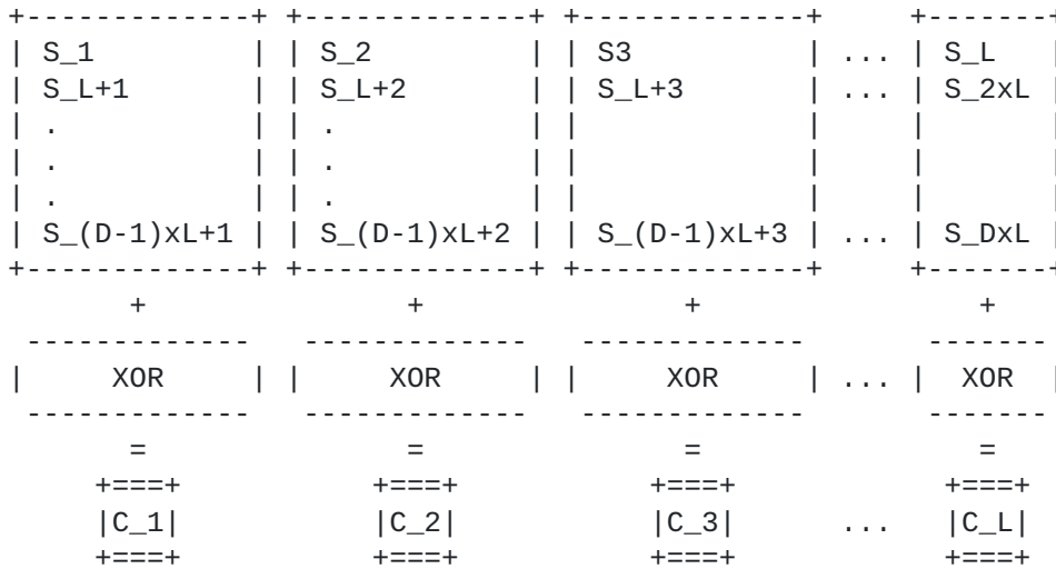
Figure 4: Generating interleaved (column) FEC repair packets
