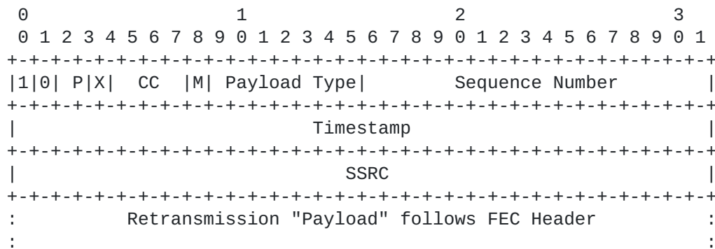
Figure 15: FEC Header for Retransmission
