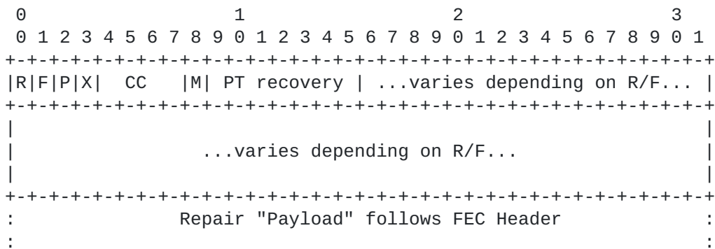
Figure 10: FEC Header
