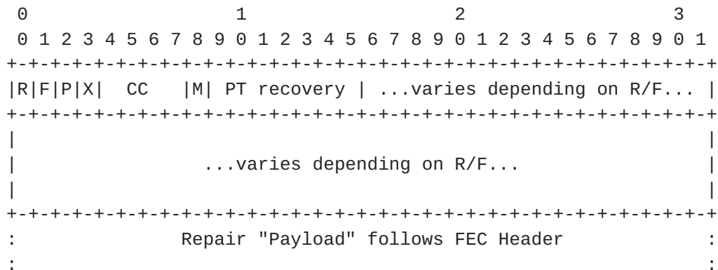
Figure 10: FEC Header
