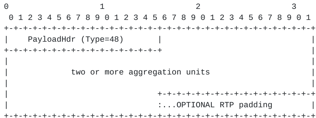
Figure 4 The structure of an aggregation packet
