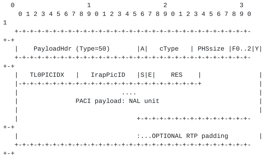
Figure 12 The structure of a PACI with a PHES containing a TSCI
