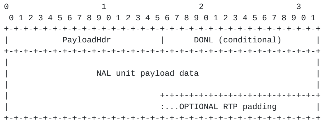
Figure 3 The structure a single NAL unit packet
