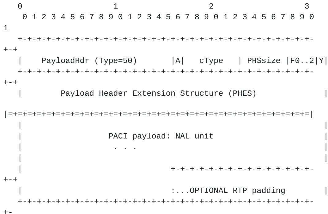
Figure 11 The structure of a PACI
