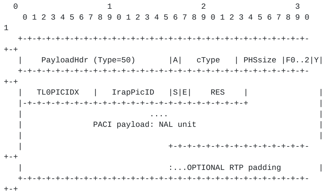
Figure 12 The structure of a PACI with a PHES containing a TSCI
