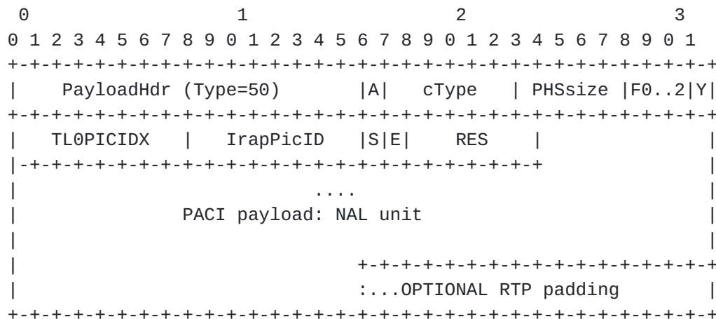
Figure 12 The structure of a PACI with a PHES containing a TSCI
