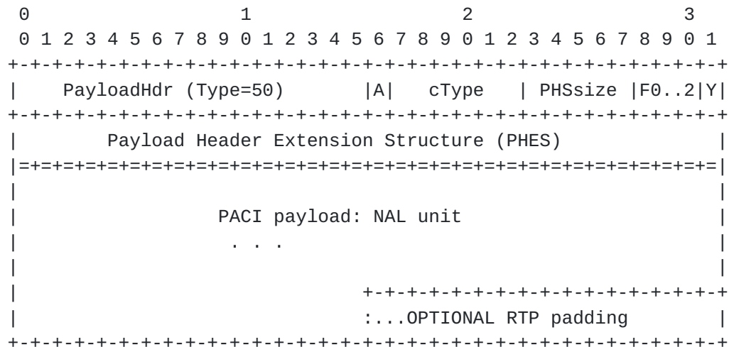
Figure 11 The structure of a PACI
