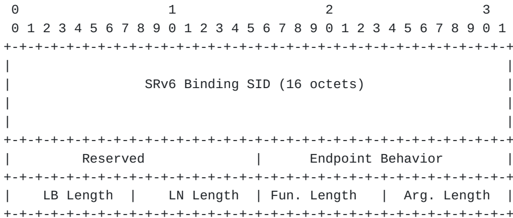
Figure 4: SRv6 Endpoint Behavior and SID Structure
