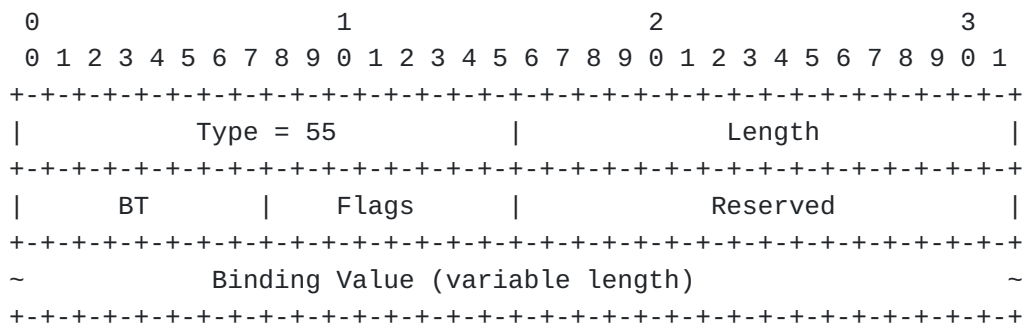
Figure 2: TE-PATH-BINDING TLV
