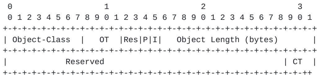
Figure 1 CLASSTYPE object format.
