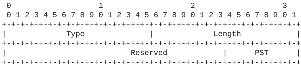
Figure 1: PATH-SETUP-TYPE TLV
