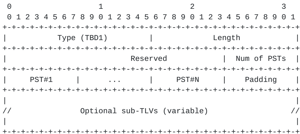
Figure 1: PATH-SETUP-TYPE-CAPABILITY TLV
