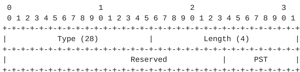
Figure 2: PATH-SETUP-TYPE TLV
