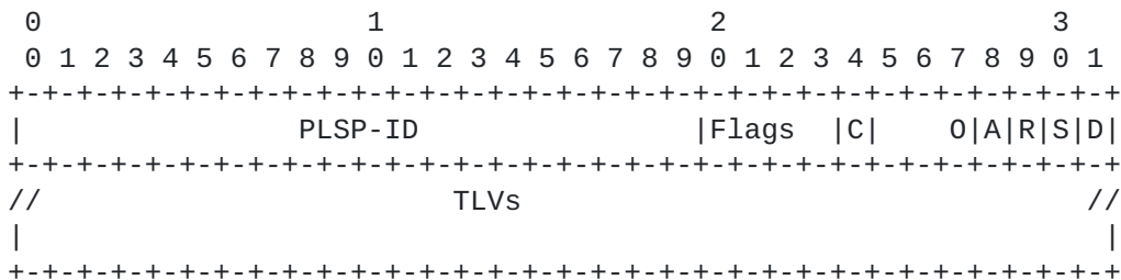
Figure 3: The LSP Object format
