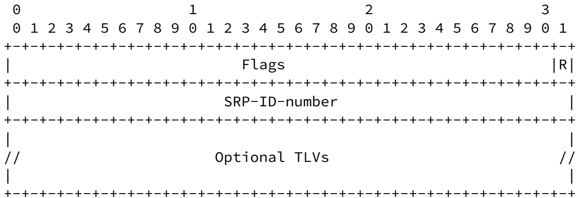
Figure 2: The SRP Object format
