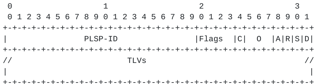
Figure 4: The LSP Object format
