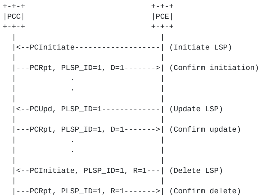
Figure 1: PCE-Initiated LSP lifecycle
