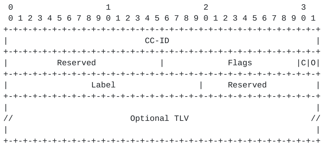
Figure 7: CCI Object
