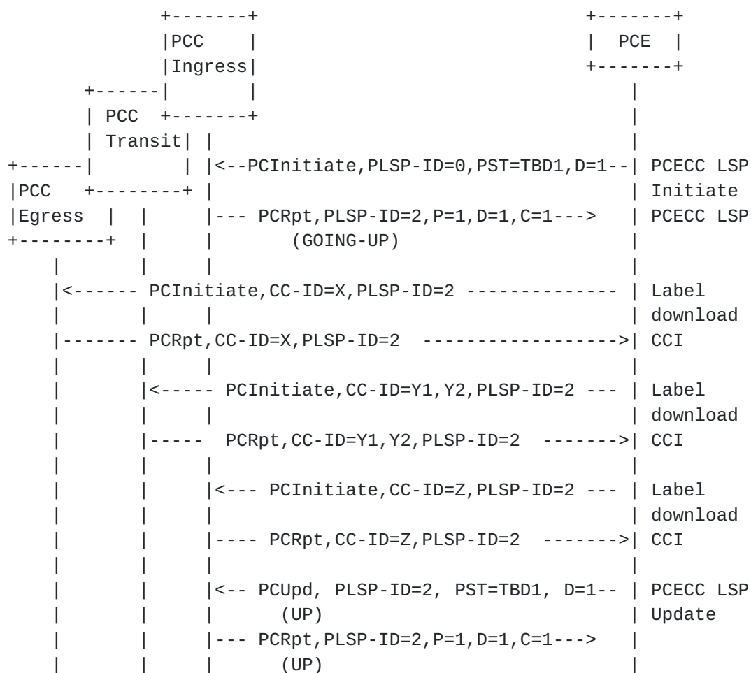
Figure 4: PCE Initiated PCECC LSP
