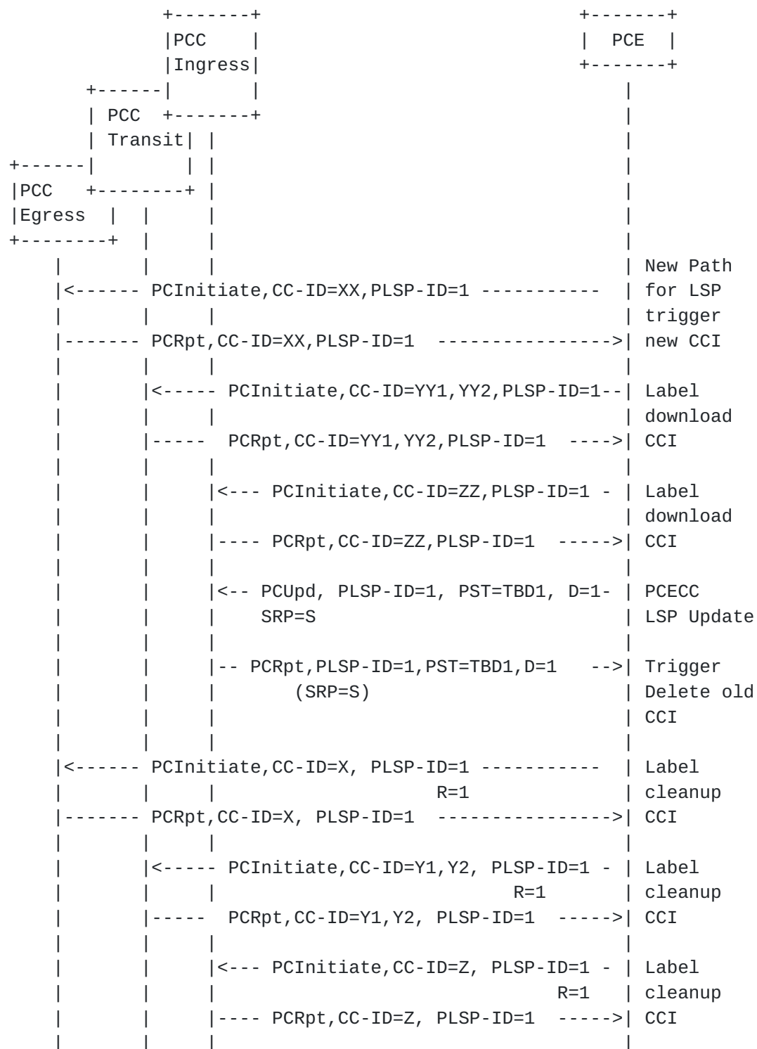
Figure 5: PCECC LSP Update
