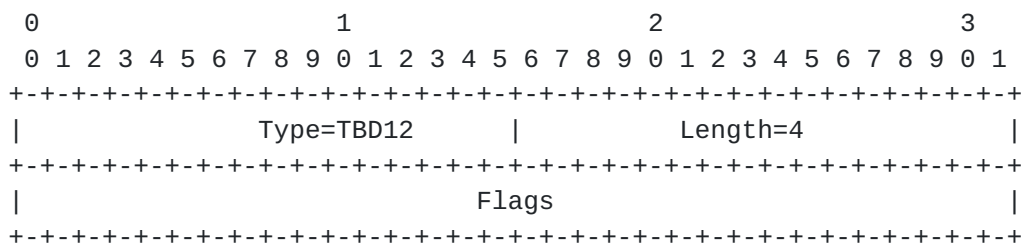
Figure 6: PCECC Capability sub-TLV
