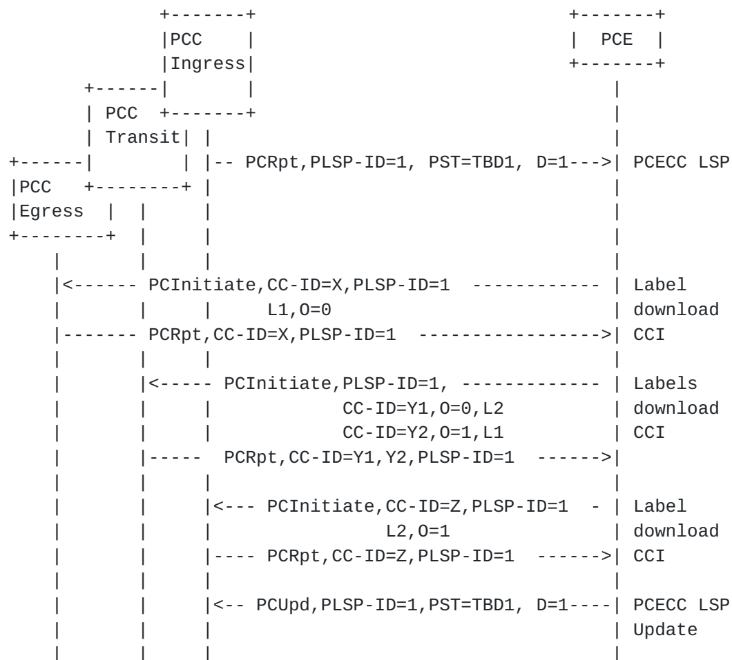
Figure 1: Basic PCECC LSP setup
