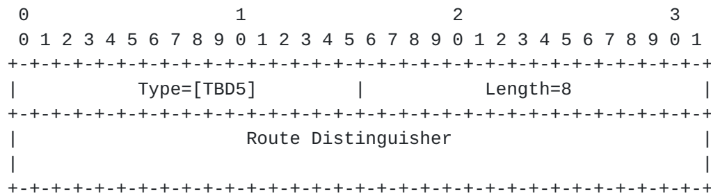
Figure 5: The Format of the ROUTE-DISTINGUISHER TLV
