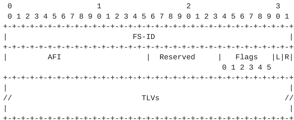
Figure 2: PCEP FLOWSPEC Object Body Format
