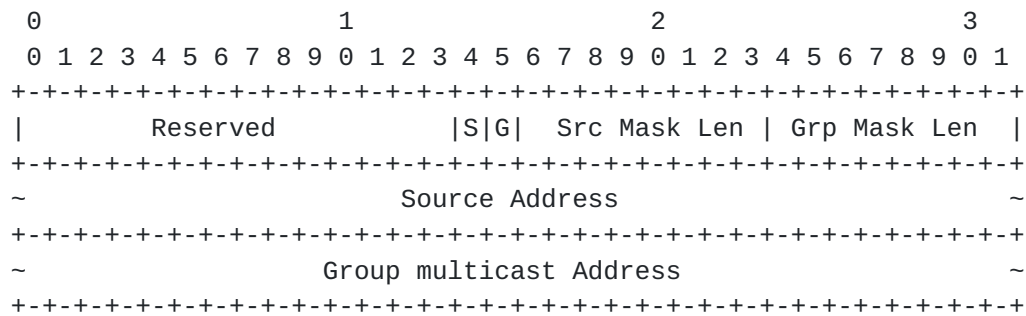
Figure 6: Multicast Flow Specification TLV Encoding
