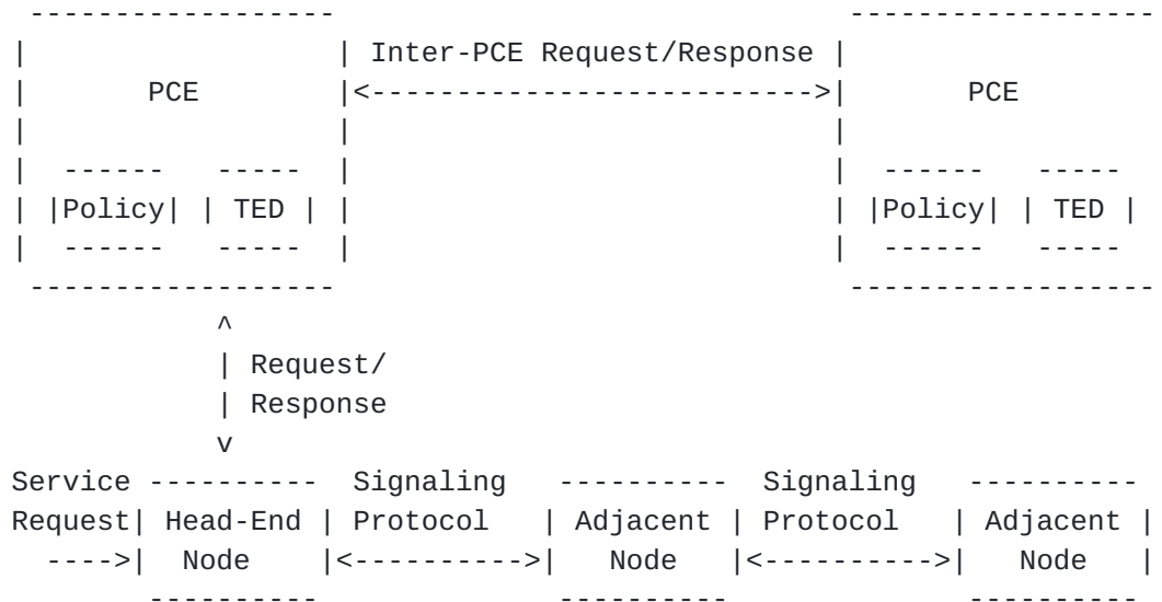
Figure 3. Multiple PCE Path Computation with Inter-PCE Communication
