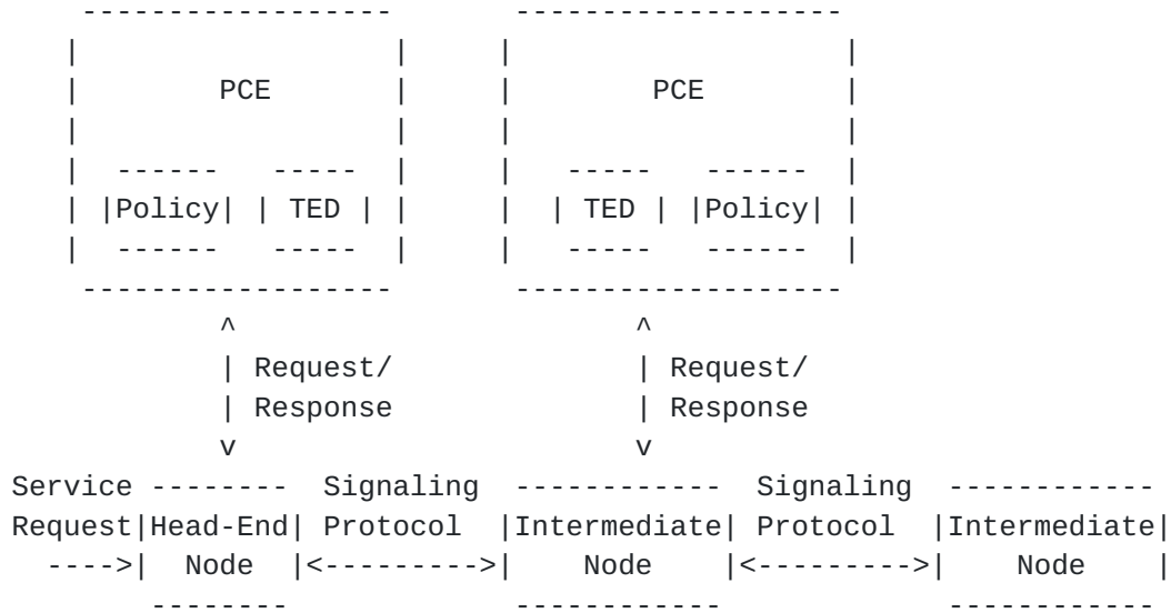
Figure 2. Multiple PCE Path Computation
