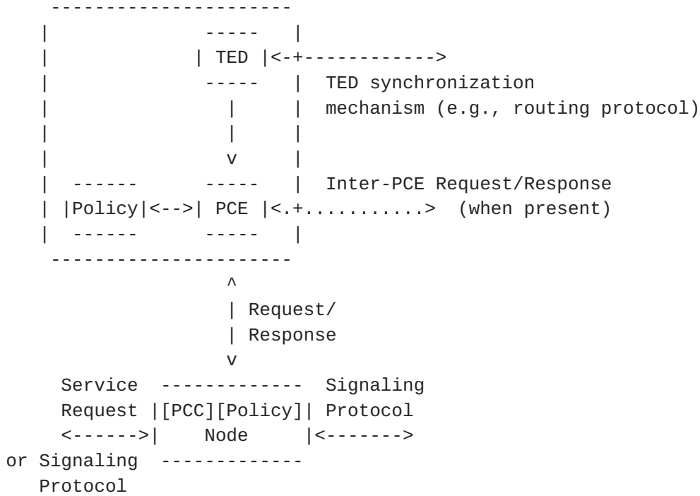
Figure 1: Policy Enabled PCC and PCE
