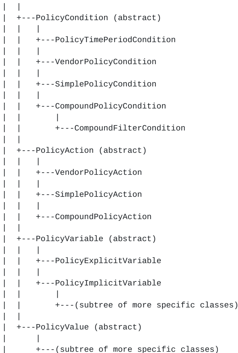
Figure 6: PCIM Class Inheritance
