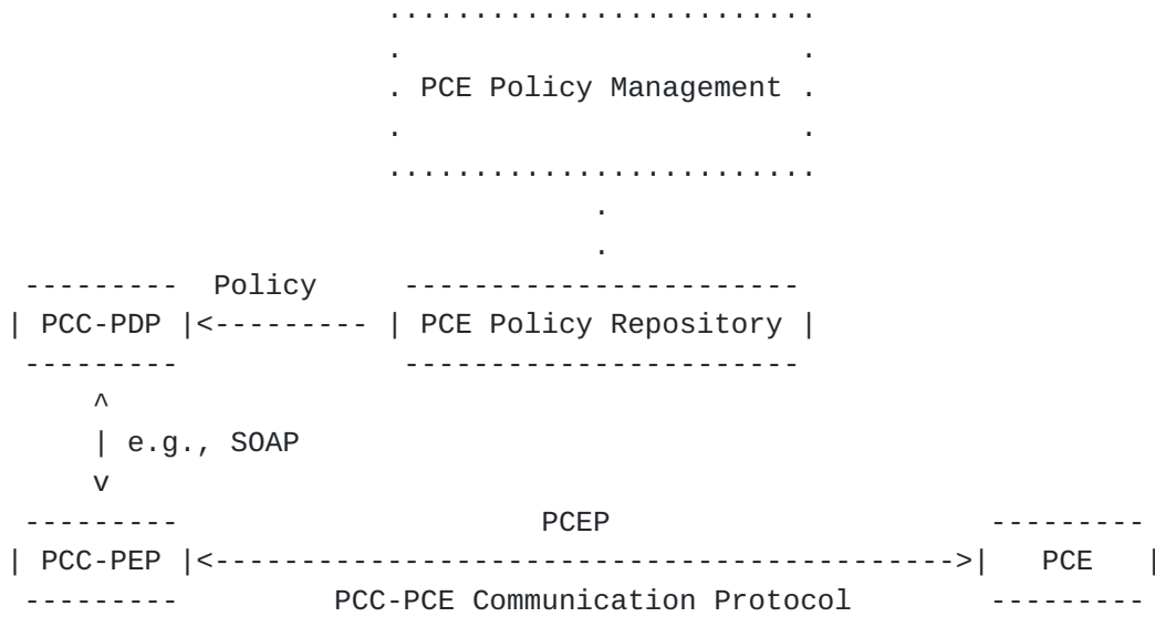
Figure 7: Policies Applied On PCC Only
