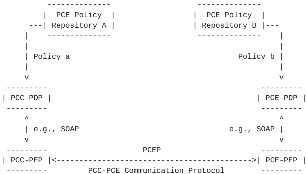
Figure 10: Multiple PCE/PCC Policy Repositories
