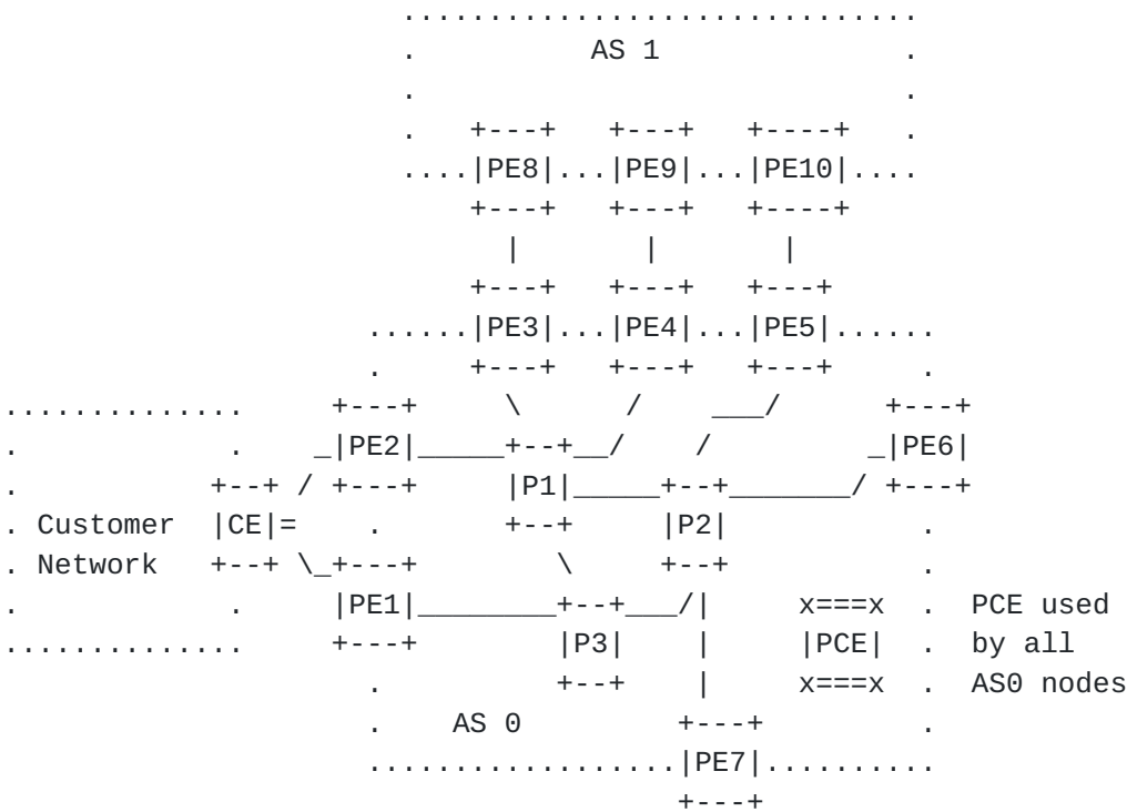
Figure 5: Advanced Load Balancing
