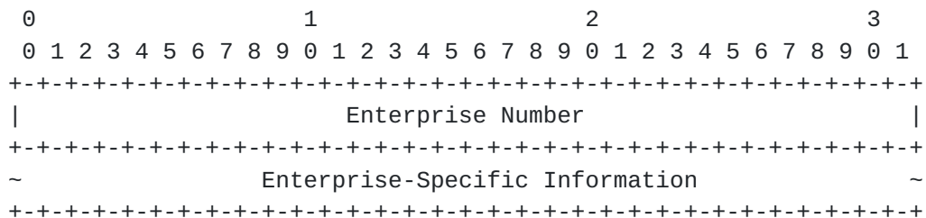
Figure 1 : Format of the Vendor Information Object and TLV
