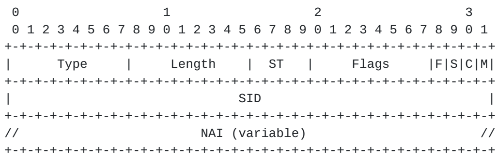
Figure 6: SR-RR0 Subobject format
