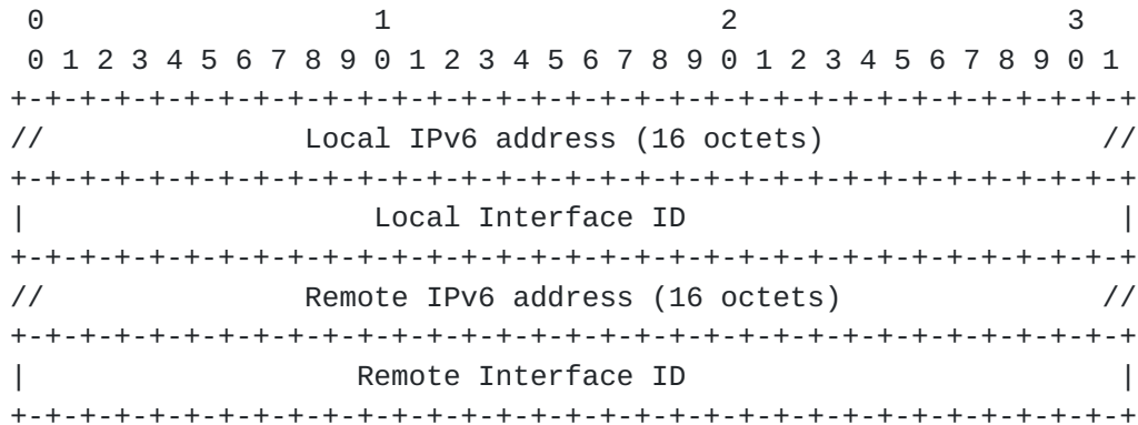
Figure 6: NAI for IPv6 link-local adjacency
