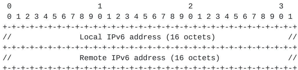
Figure 4: NAI for IPv6 global adjacency
