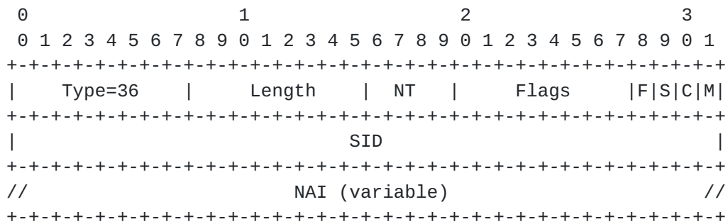
Figure 7: SR-RR0 Subobject format
