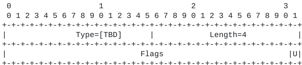
Figure 9: STATEFUL-PCE-CAPABILITY TLV format
