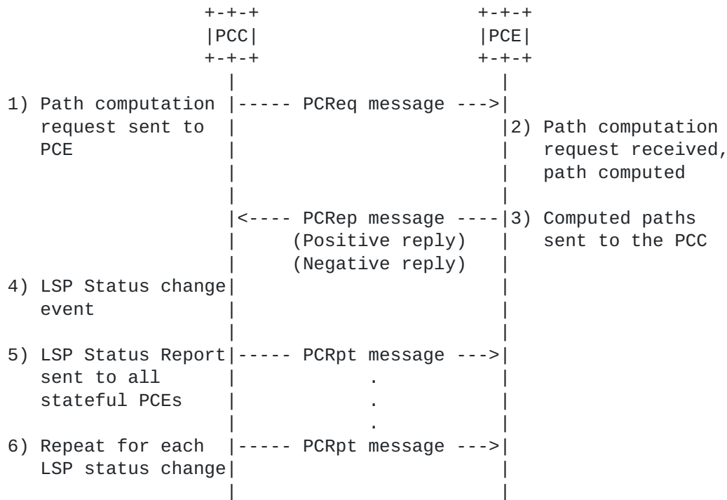
Figure 7: Passive Stateful PCE Path Computation Request/Response
