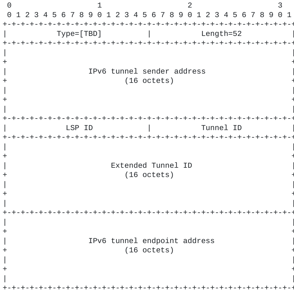
Figure 13: IPV6-LSP-IDENTIFIERS TLV format
