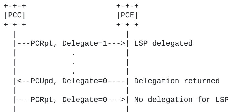
Figure 6: Returning a Delegation
