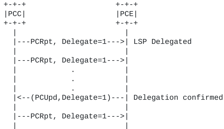
Figure 4: Delegating an LSP
