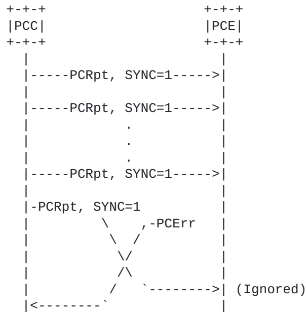
Figure 2: Failed state synchronization (PCE failure)
