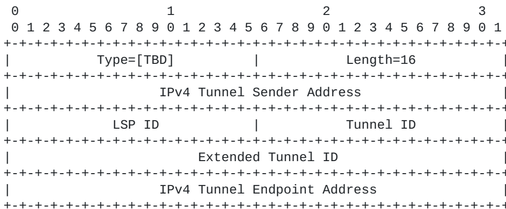
Figure 12: IPV4-LSP-IDENTIFIERS TLV format
