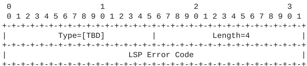
Figure 15: LSP-ERROR-CODE TLV format
