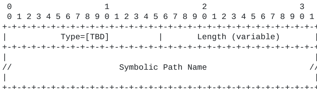
Figure 14: SYMBOLIC-PATH-NAME TLV format
