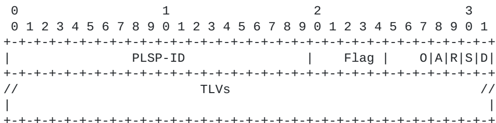
Figure 11: The LSP Object format
