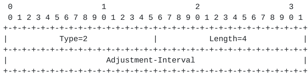
Adjustment-Interval sub-TLV format
