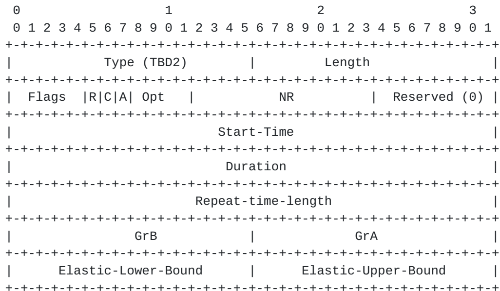
Figure 2: SCHED-PD-LSP-ATTRIBUTE TLV
