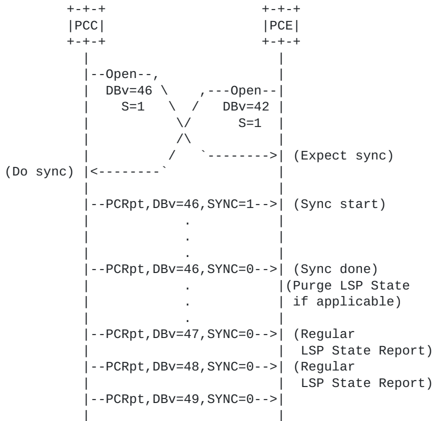
Figure 2: State Synchronization Performed
