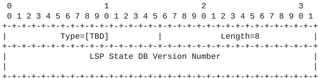
Figure 4: LSP-DB-VERSION TLV format
