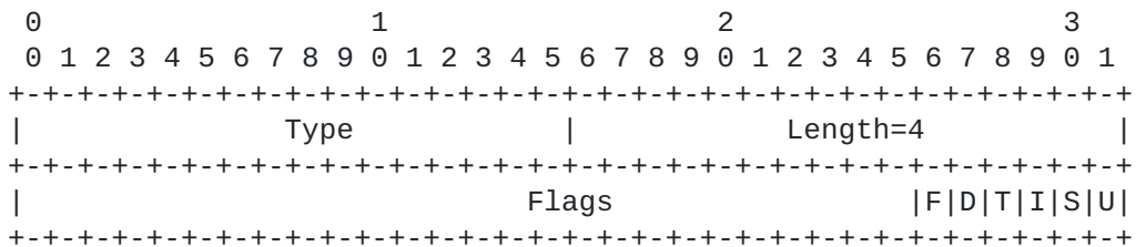
Figure 8: STATEFUL-PCE-CAPABILITY TLV Format
