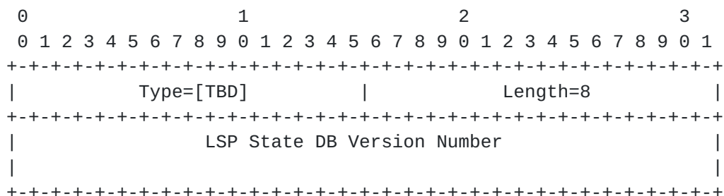
Figure 4: LSP-DB-VERSION TLV format
