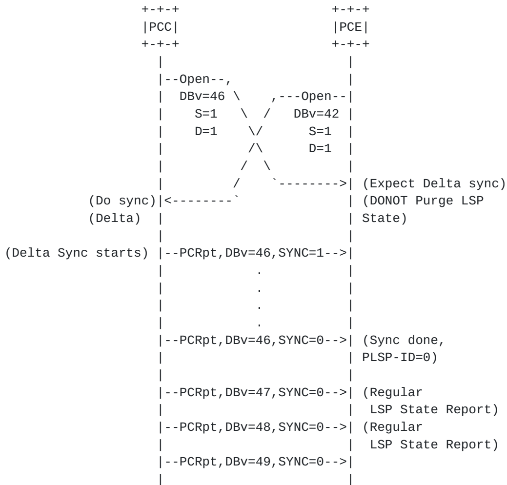
Figure 7: Incremental Synchronization Procedure
