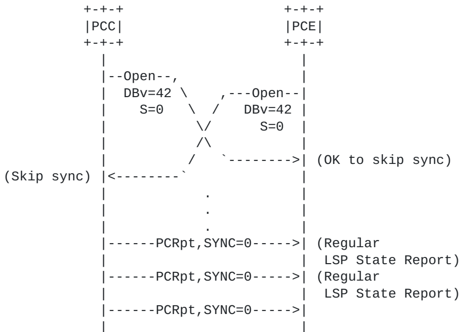
Figure 3: State Synchronization Skipped, no LSP-DB-VERSION TLVs sent from PCC
