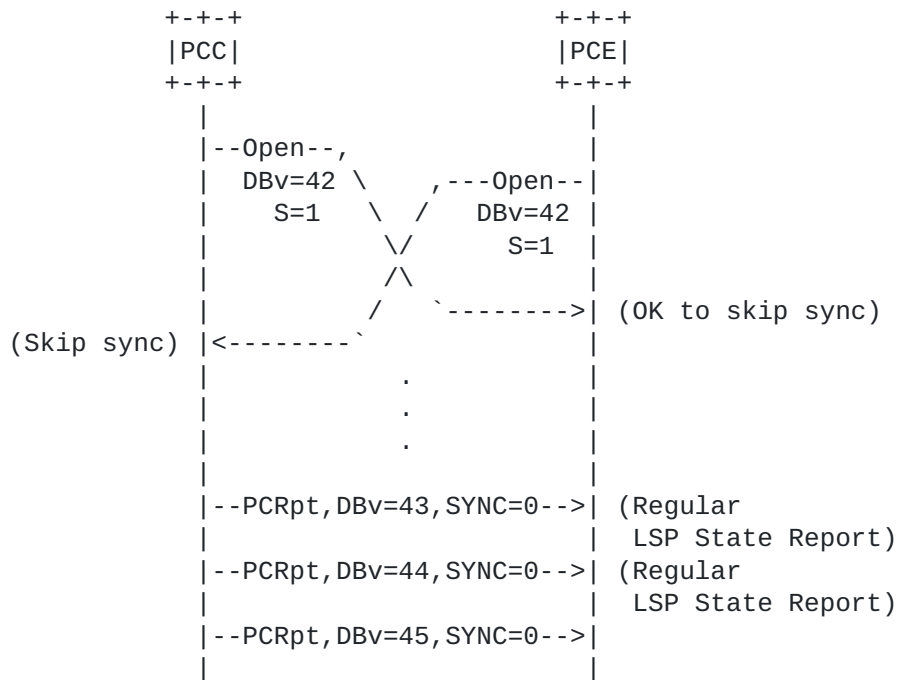
Figure 1: State Synchronization Skipped
