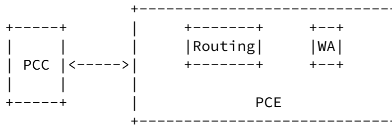
Figure 2 Combined Process (R&WA) architecture
