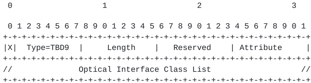
Figure 5 Optical Interface Class List XRO Subobject
