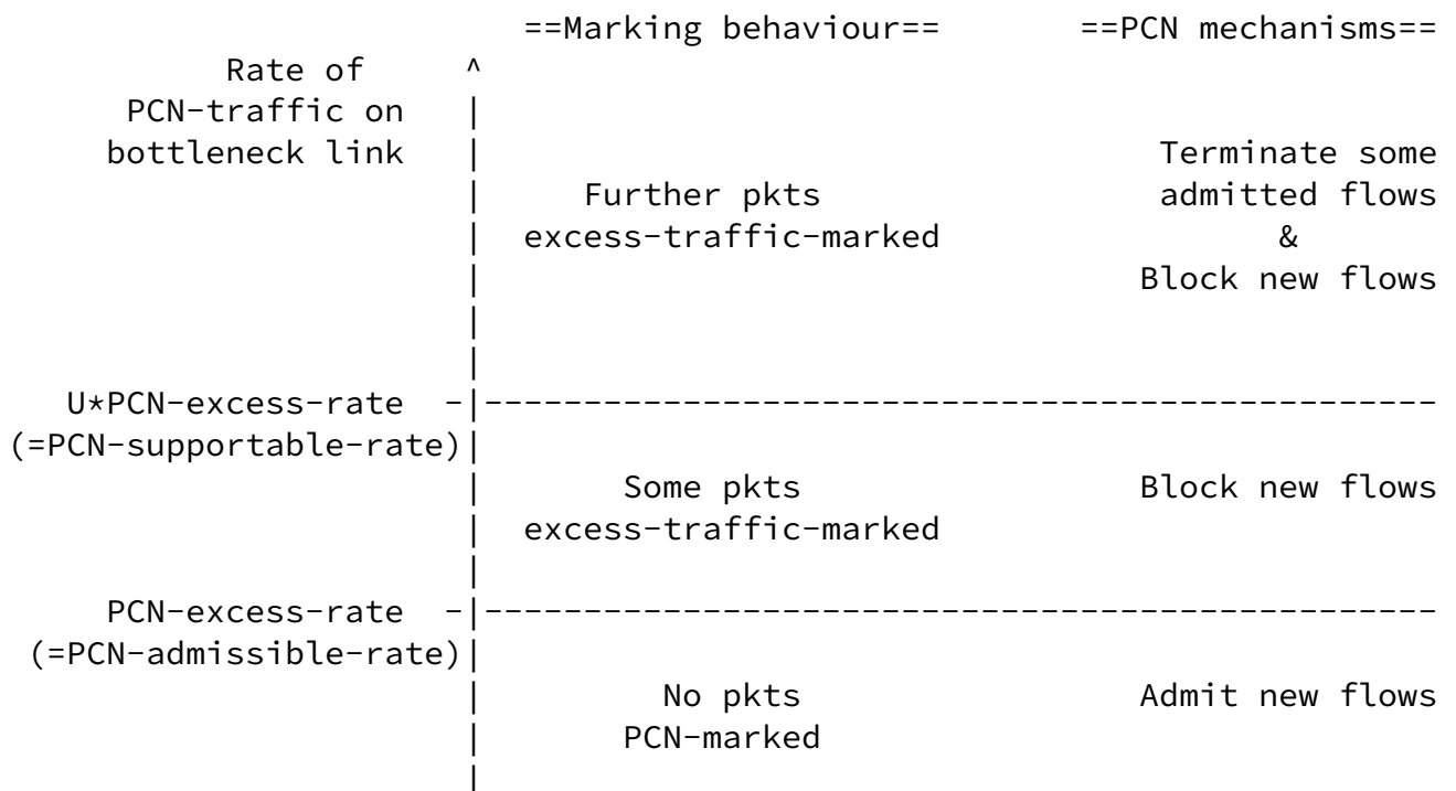
Figure 2: Schematic of how the PCN admission control and flow termination mechanisms operate as the rate of PCN-traffic increases,
