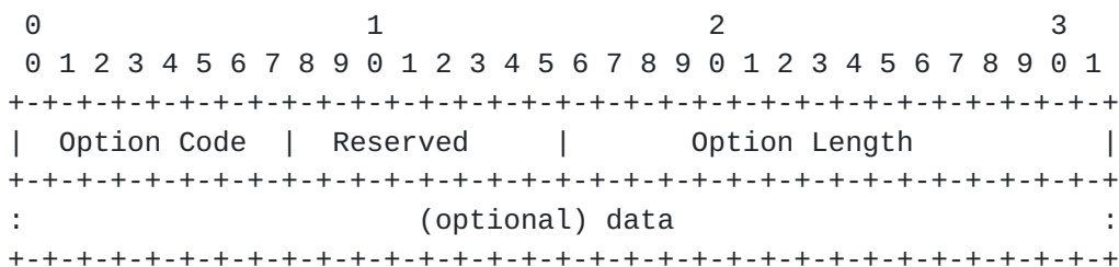
Figure 4: Options Header
