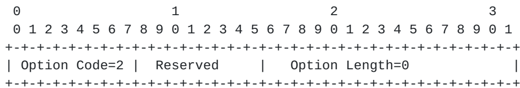
Figure 14: PREFER_FAILURE Option
