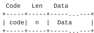
Figure 3: PCP Server sub-option
