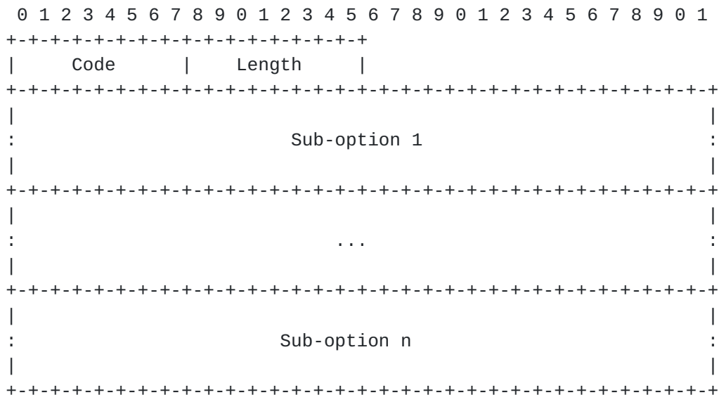
Figure 2: IPv4 DHCP PCP Option
