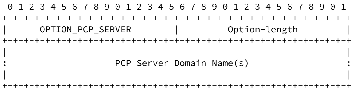
Figure 1: PCP Server Name DHCPv6 Option
