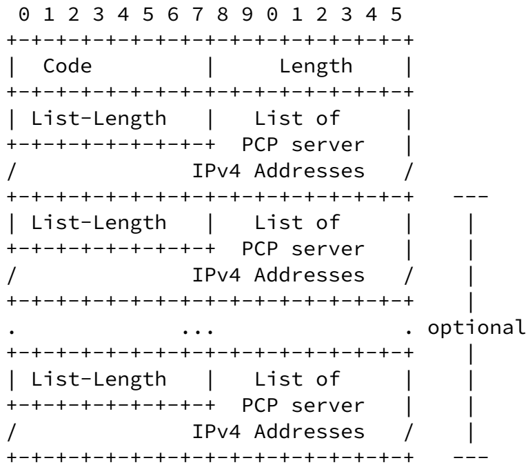
Figure 2: DHCPv4 PCP server option
