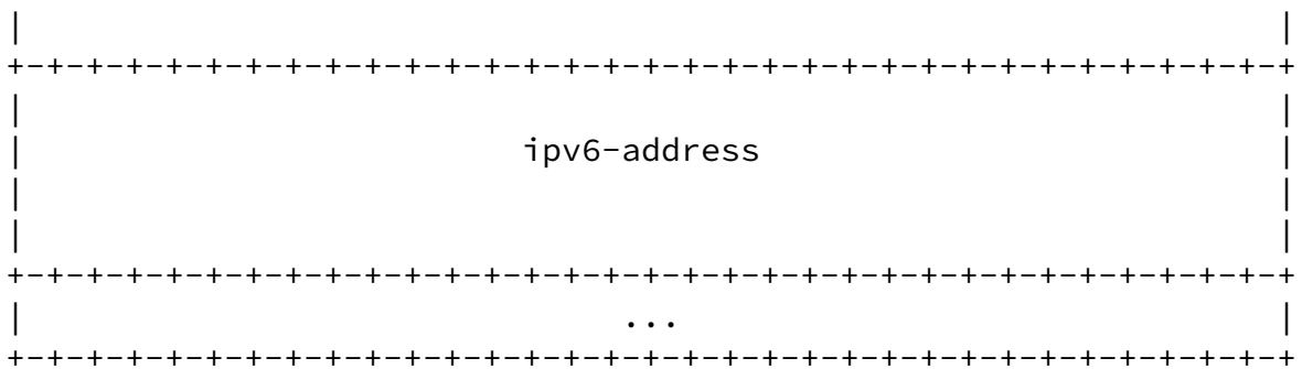
Figure 1: DHCPv6 PCP server option
