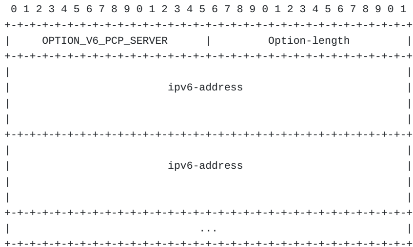
Figure 1: DHCPv6 PCP server option
