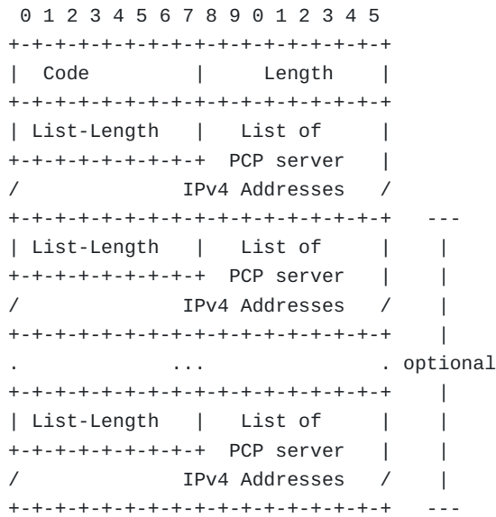
Figure 2: DHCPv4 PCP server option
